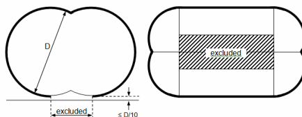
Bilobe tanks
